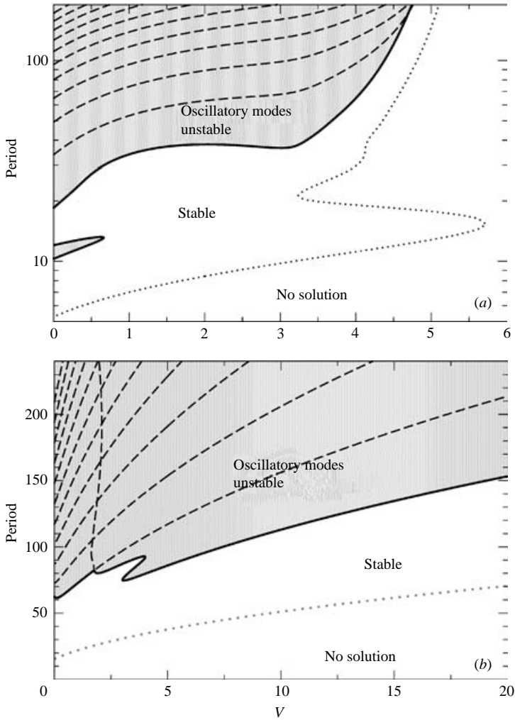
FIGURE 13. The linear stability of n=1 stationary solutions of different periods as a function of the vibration number V for (a) \alpha = 0.19 and (b) \alpha = 0.4 . The solid lines delimit the instability region (shaded) and correspond to stationary instability in the comoving frame. The dashed lines indicate the location of subsequent oscillatory instabilities. The dotted line in (a) indicates the locus of the saddle-node bifurcations at which the primary branch acquires stability, while the dotted line in (b) corresponds to the primary (supercritical) bifurcation. Thus in (b) n=1 solutions exist only above the dotted line. The parameters are G = 1.0 , Bi = 0.5 , M = 3.5 .
